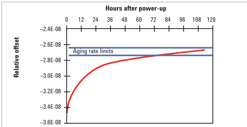
Figure 2. A representation of the warm-up characteristic of a high stability, ovenized quartz crystal oscillator. In this example the drift or aging rate specification is 1 part in 10^9 per day.
