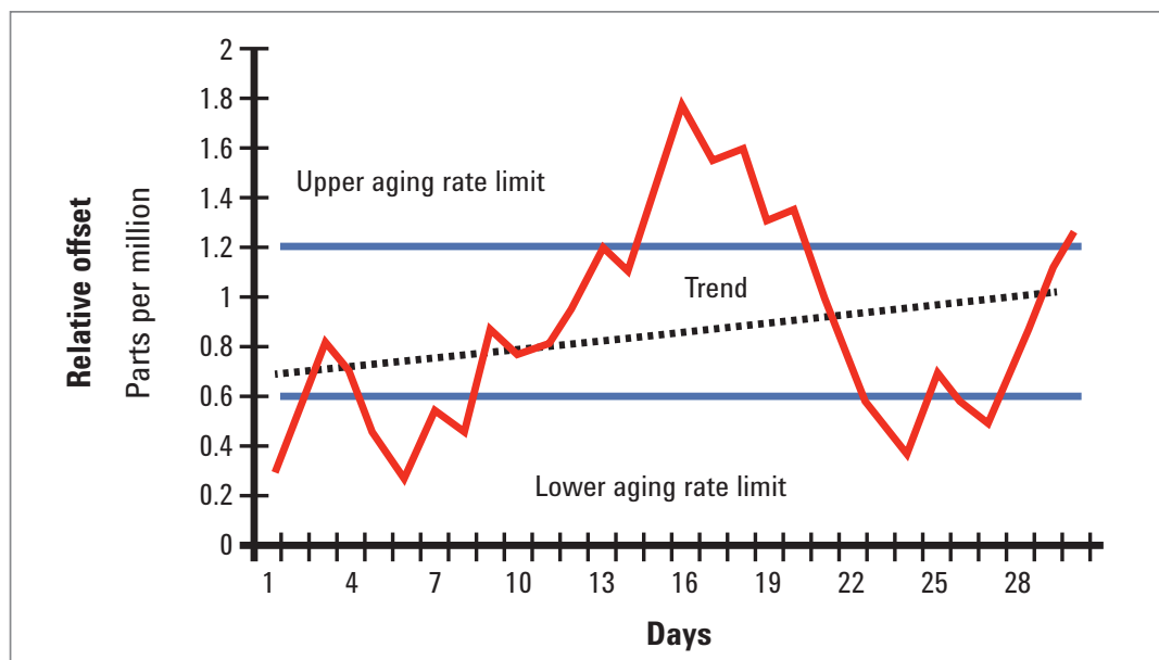
Figure 1. A representation of the frequency stability of an uncompensated or temperature compensated quartz crystal oscillator. Note how the aging rate would far exceed, or be far less than, specification if measurements were taken over a shorter period than the specified one month for this oscillator. The apparent aging rate would also vary considerably depending when the measurements were made.
